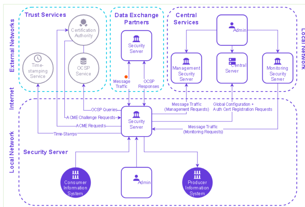
Figure 20 - X-Road Architecture
