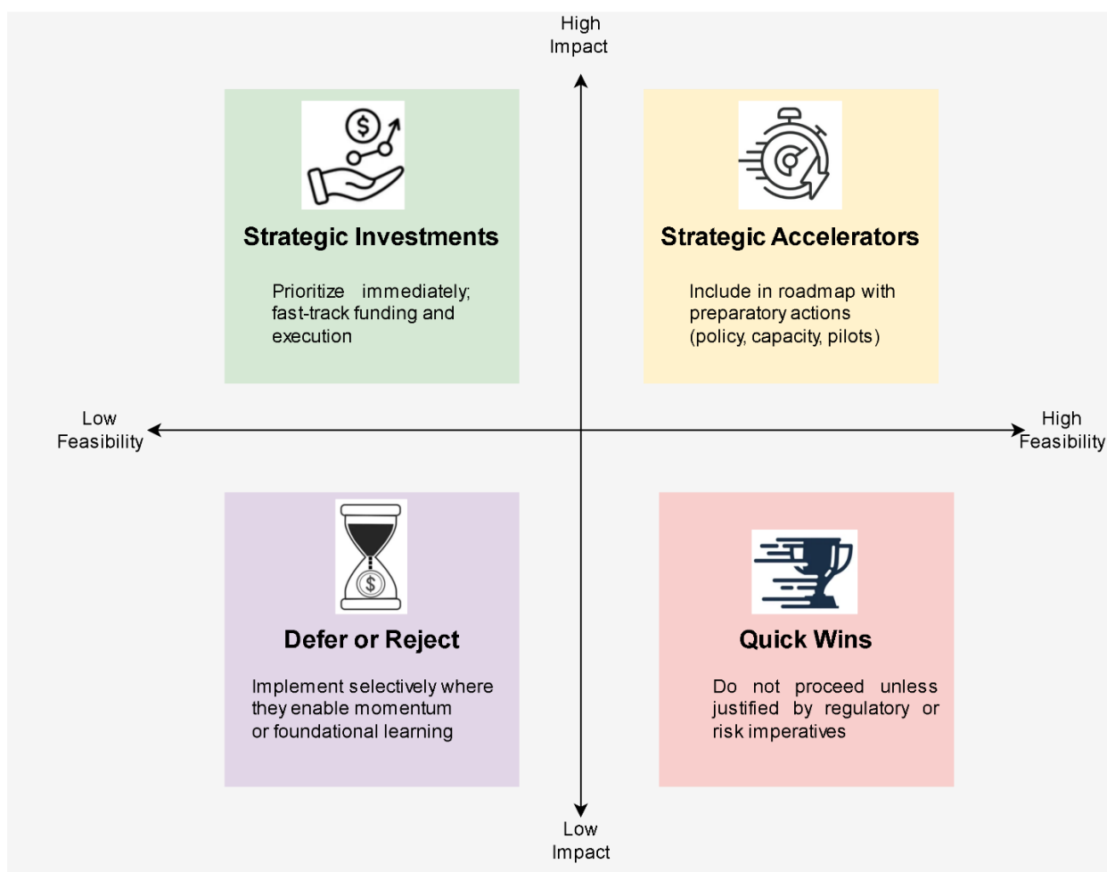
Figure 30- Impact-Feasibility Matrix
